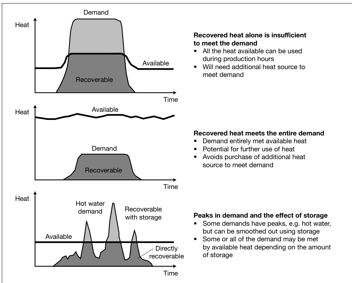
Fig 10 Matching heat demand and heat availability
