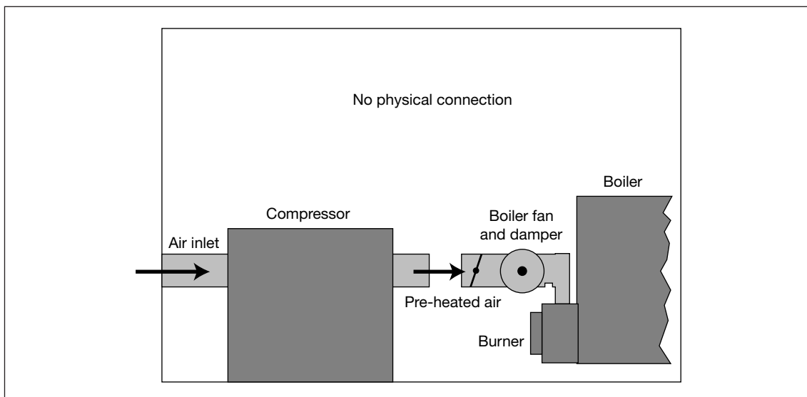
Fig 9 Indirect boiler intake of hot air
