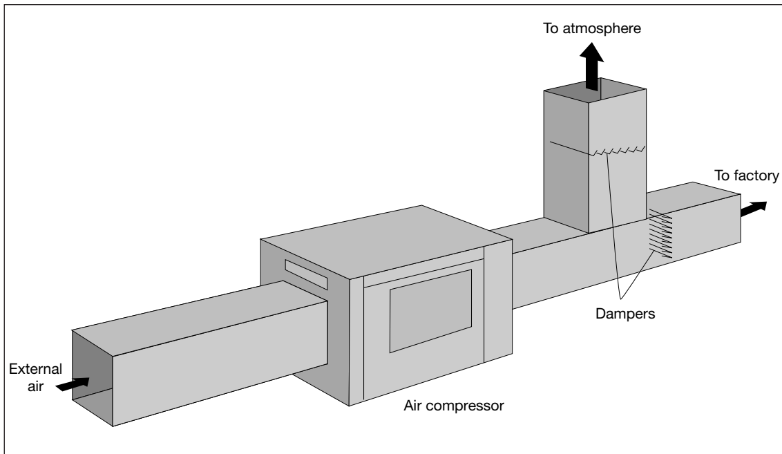
Fig 5 Typical large air-cooled compressor with direct heat recovery
