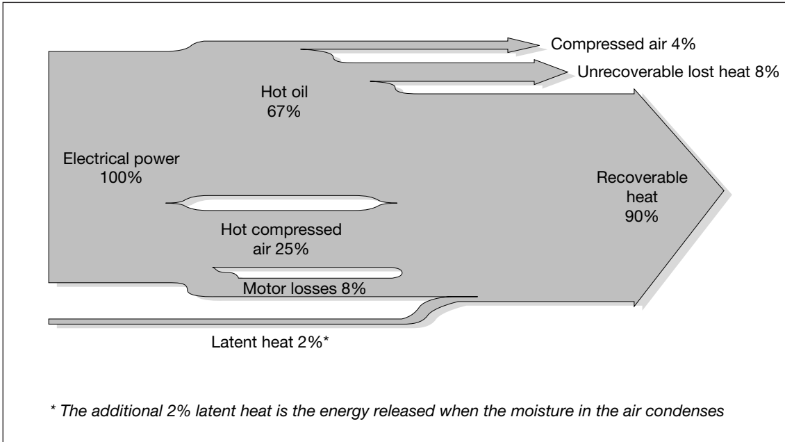
Fig 1 Energy flow in a typical oil-injected screw compressor
