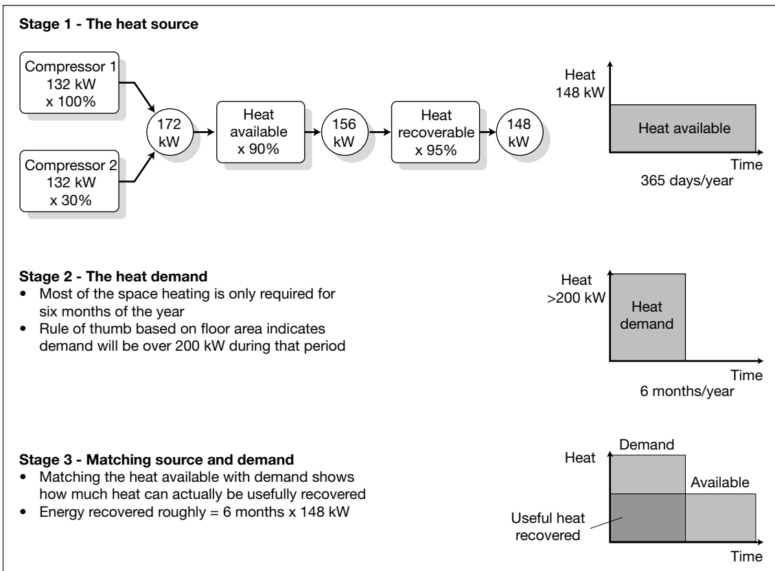
Fig 11 Example of matching source and demand
