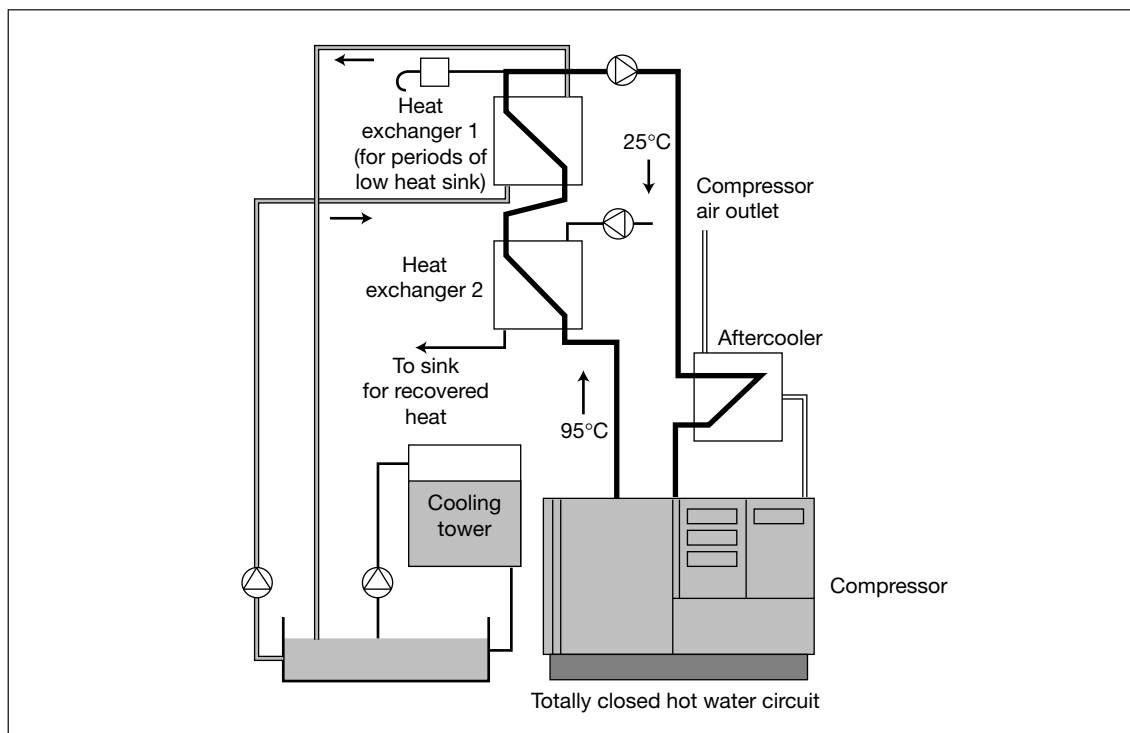
Fig 7 A sophisticated oil-to-water heat recovery system
